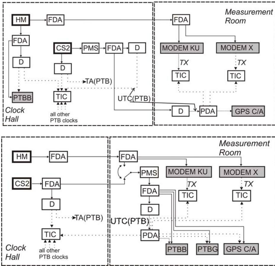
Figure 3. Realization of UTC (PTB); upper graph: arrangement in service until September 2003, lower graph: new arrangement. HM: hydrogen maser, FDA: frequency distribution amplifier, D: divider delivering 1 PPS signals, TIC: time interval counter, PDA: pulse distribution system, PMS: phase micro stepper. Solid lines: 5 MHz signals, dotted lines: 1 PPS signals, gray boxes: time transfer equipment, mentioned in the text. Frequency converters (e.g. 5 MHz to 10 MHz or 20 MHz) are not shown.
