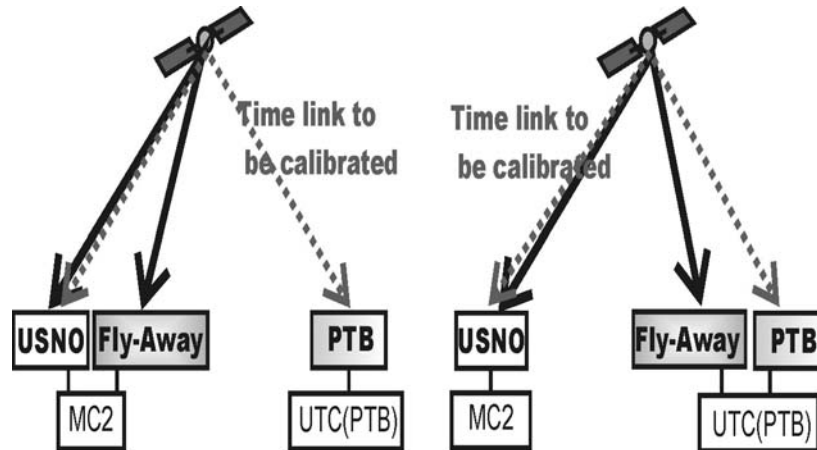
Figure 8. Schematic representation of the setup of a travelling TWSTFT station sequentially at USNO and PTB. The stations are given as gray shaded squares. The solid arrows indicate the time transfer performed during the measurement campaigns. The dashed lines indicate time transfer links that can in principle be calibrated that way.
