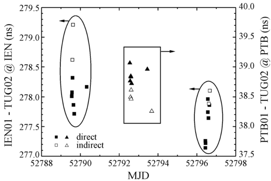
Figure 5. Results of differential delay measurements of the pairs of TWSTFT stations IEN01, PTB01 and TUG02, operated in sequence at IEN (labeled IEN01-TUG02, left axis, squares) and PTB (labeled PTB01-TUG02, right axis, triangles), as explained in the text. Full symbols: direct measurement, open symbols: indirect measurements (see Fig. 4 for explanation). Data were taken from [9].
