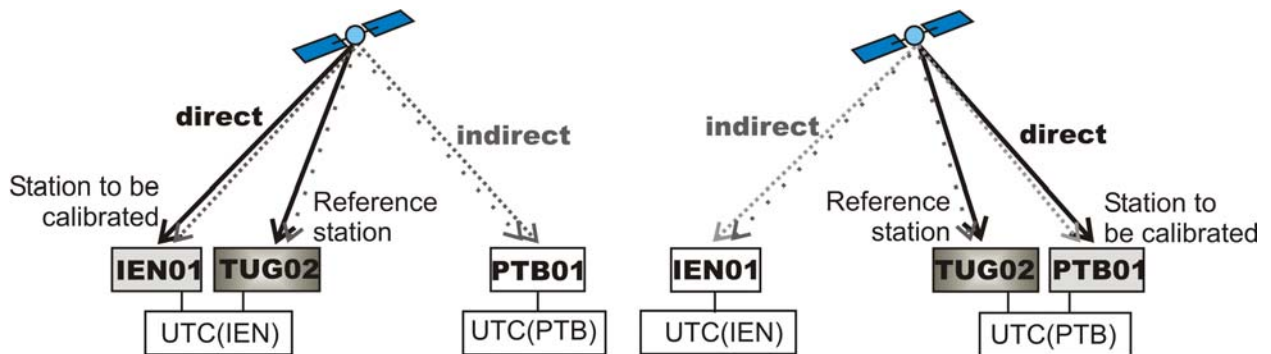
Figure 4. Schematic representation of the setup of a travelling TWSTFT station sequentially at IEN, Torino, and PTB. The TWSTFT stations are given as gray shaded squares. The solid arrows represent the direct time transfer performed during the measurement campaigns. The dashed arrows indicate the additionally evaluated links that give so-called indirect results.
